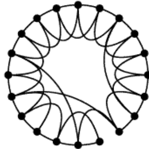
Small-world
