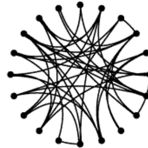
Random
